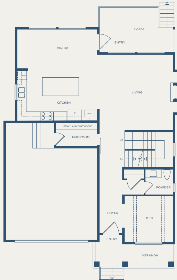
MAIN 1,153 SQFT
